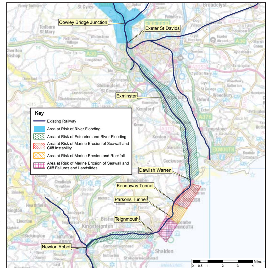
Figure 2: Geo-environmental threats to the Exeter to Newton Abbot railway
